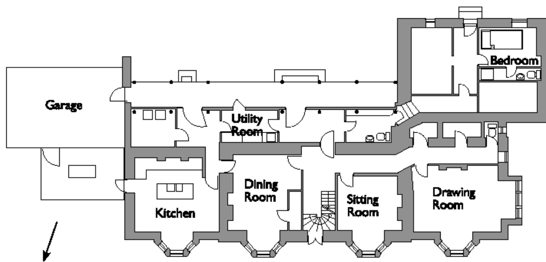
Kindrochet Ground Floor
